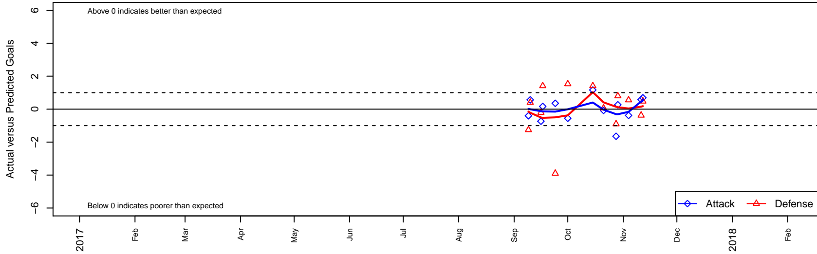
NEU Blue G04 Dots are actual minus expected GF (blue circles) and GA (red triangles). Blue line is smoothed change in attack strength. Red is smoothed change in defense strength.
